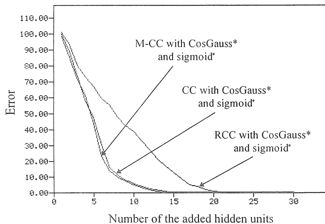
Fig 13: Comparison of the error curve between the CC-, RCC and M-CC network using the CosGauss activation function for the candidate and the hidden units.
