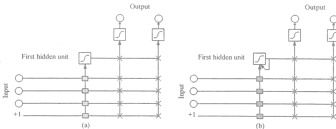
Fig. 3: First generation of the modified Cascade Correlation network: (a): with a feedforward unit and (b): with a recurrent unit.
