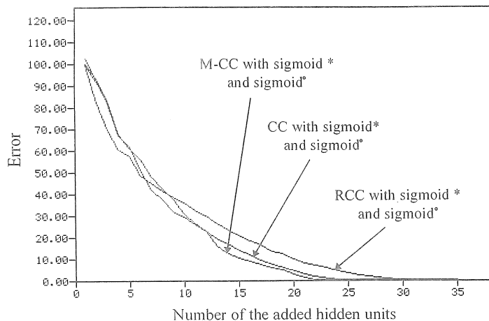
Fig 7: Comparison of the error curve between the CC-, RCC and M-CC network using the sigmoid activation function for the candidate and the hidden units.
