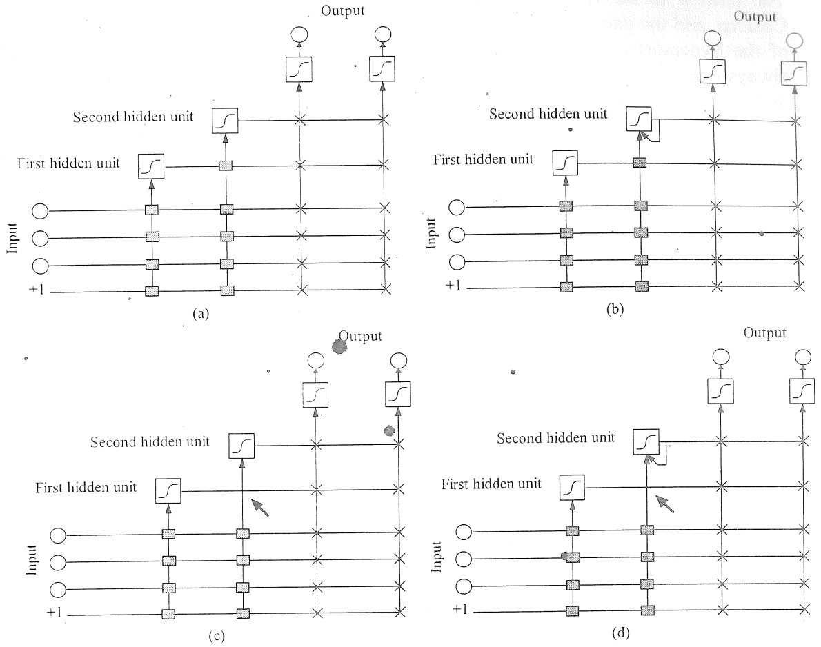
Fig. 4: Second generation of the modified Cascade Correlation network: (a): vertical growth, feedforward, (b): vertical growth, recurrent, (c): horizontal growth, feedforward, (d): horizontal growth, recurrent.
