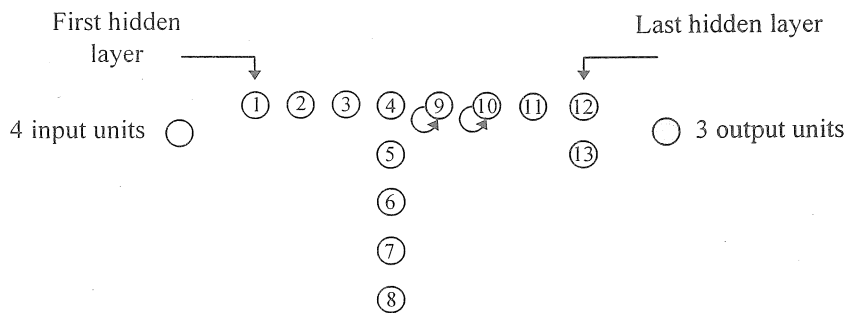
Fig. 12: Arrangement of the created hidden units on the hidden layers of the trained M-CC network using CosExp activation function for the candidate and the hidden units.
