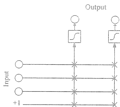
Fig. 2: Initialization of the modified Cascade Correlation network
