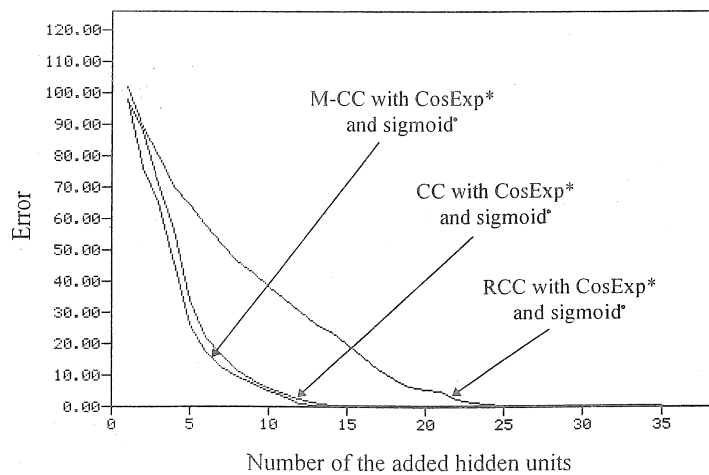
Fig 11: Comparison of the error curve between the CC-, RCC and M-CC network using the CosExp activation function for the candidate and the hidden units.
