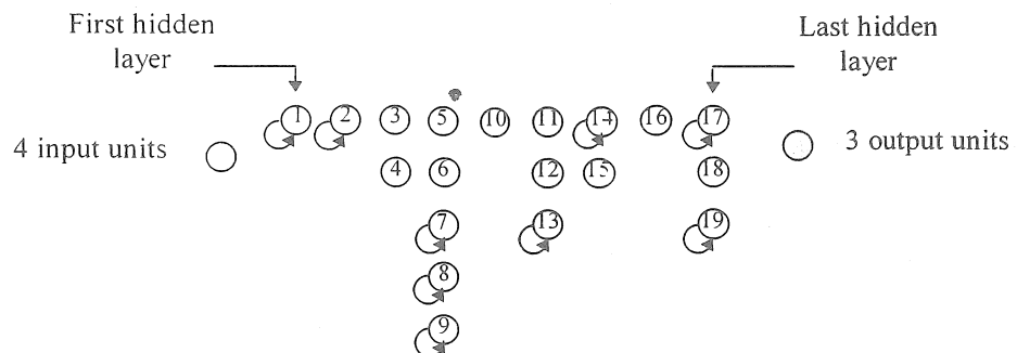
Fig. 10: Arrangement of the created hidden units on the hidden layers of the trained M-CC network using tanh activation function for the candidate and the hidden units.
