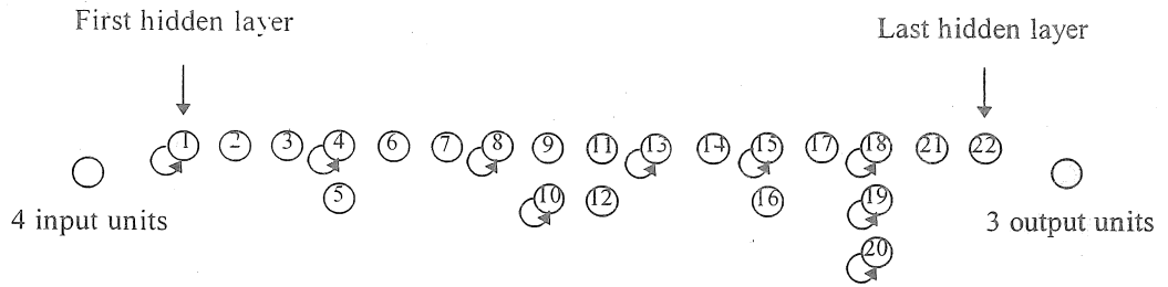
Fig. 8: Arrangement of the created hidden units on the hidden layers of the trained M-CC network using sigmoid activation function for the candidate and the hidden units.
